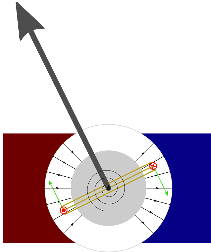
Schematic representation of a moving-coil instrument.
