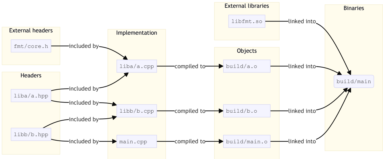
Figure 1: Dependencies between files used during the build process.
